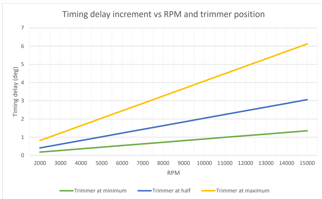
Figure 3: Timing delay introduced by the trimmer
